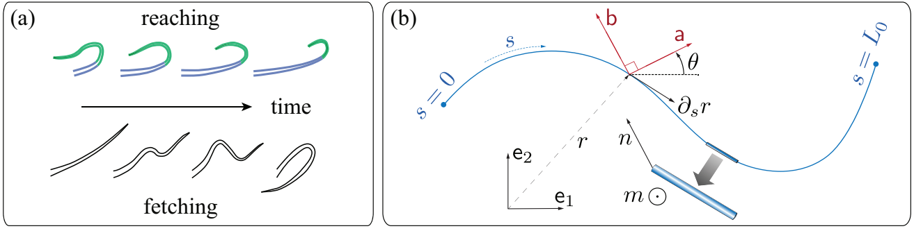
Fig. 1: (a) The octopuses have been observed to exhibit bend propagation (for reaching) and elbow formation (for fetching). The bend propagation is actively achieved by propagating muscle actuation, illustrated by blue color; green represents the unactuated portion of the arm. (b) A schematic of the planar Cosserat rod model.
