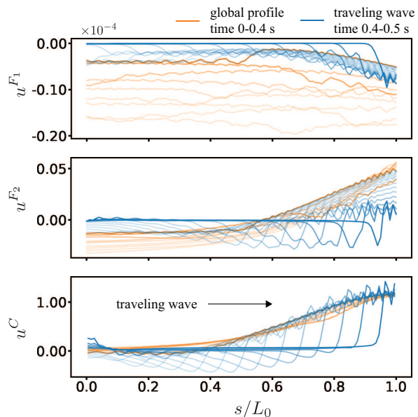
Fig. 3: Learned optimal controls for the reaching task: Control inputs u^F = (u^{F_1}, u^{F_2}) and u^C along the arm are illustrated for the last iteration. Nine time snapshots are shown in orange from t = 0 s to t = 0.4 s, and sixteen time snapshots are shown in blue from t = 0.4 s to t = 0.5 s (the most transparent lines correspond to the beginning of the time interval). The orange lines indicate the global profile of the optimal controls. The blue lines indicate the distinguishable traveling waves in optimal controls.
